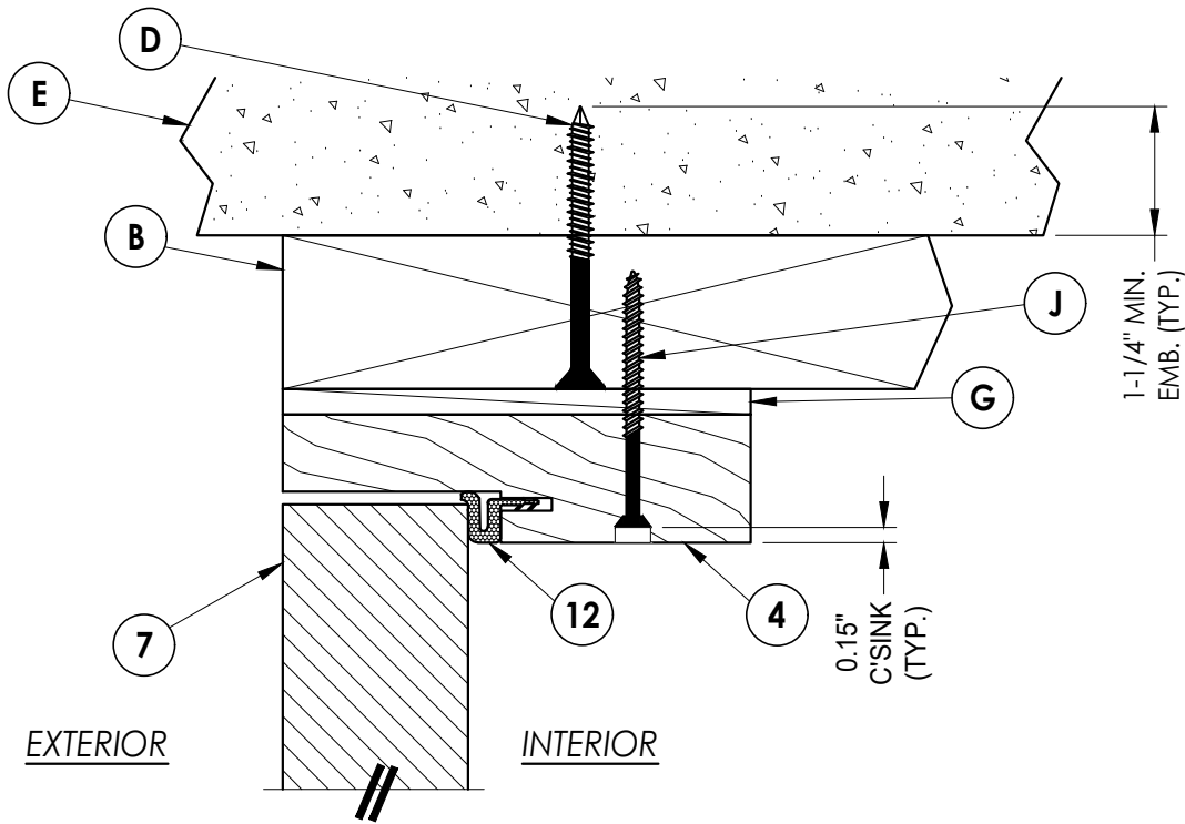
1 5 VERTICAL CROSS SECTION Outswing shown
